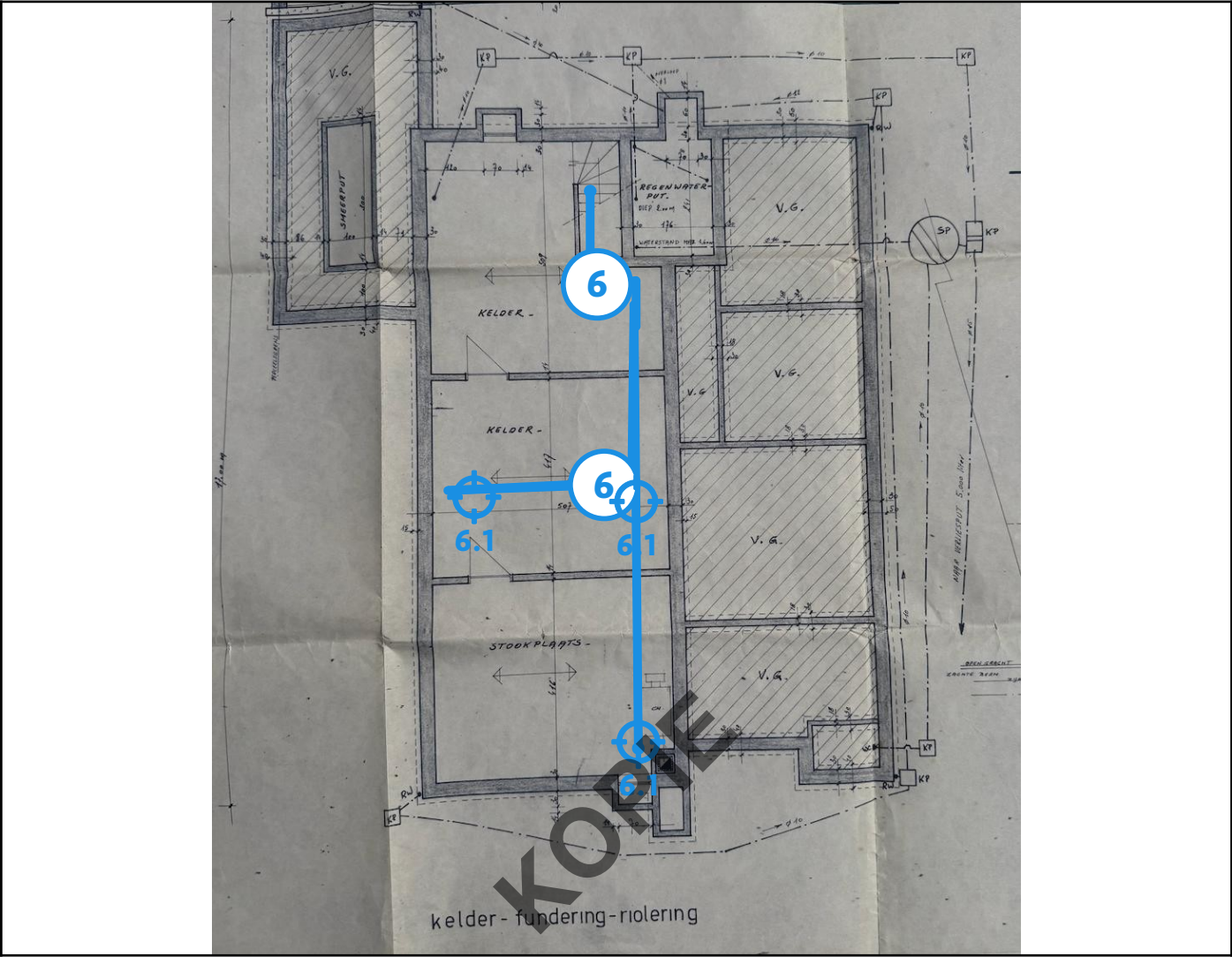
Legende van plan 1.1: Fundering/Kelder
